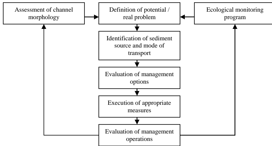
Figure 1. A holistic management framework for evaluating the effects of sediment accumulation in rivers (from Wood & Armitage, 1997).
