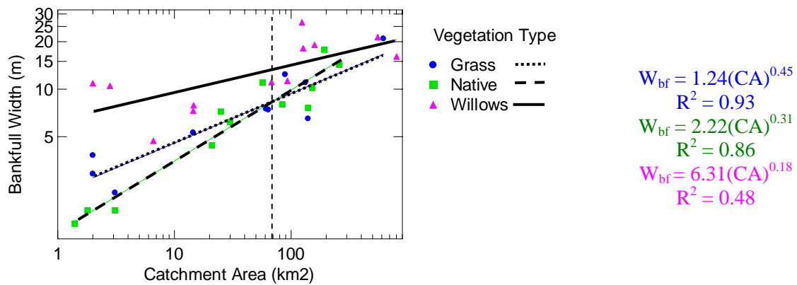
Figure 1. Scatter plot and regression equations showing the relationship between vegetation type (willows, natives or grass), bankfull width and catchment area (log-log scale). The vertical dashed line indicates the point at which sites with natives become narrower than those with grass (~60km 2 ).
