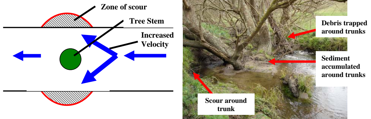
Figure 3. (a) Diagram showing how flow accelerates around mid-channel vegetation leading to bank scour (Diagram adapted from Trimble, 2004, p.155), and (b) a typical in-channel bed willow from one of the field sites (Coal Creek). Note the considerable blockage of the channel by the willow tree and the associated trapped sediment and debris.
