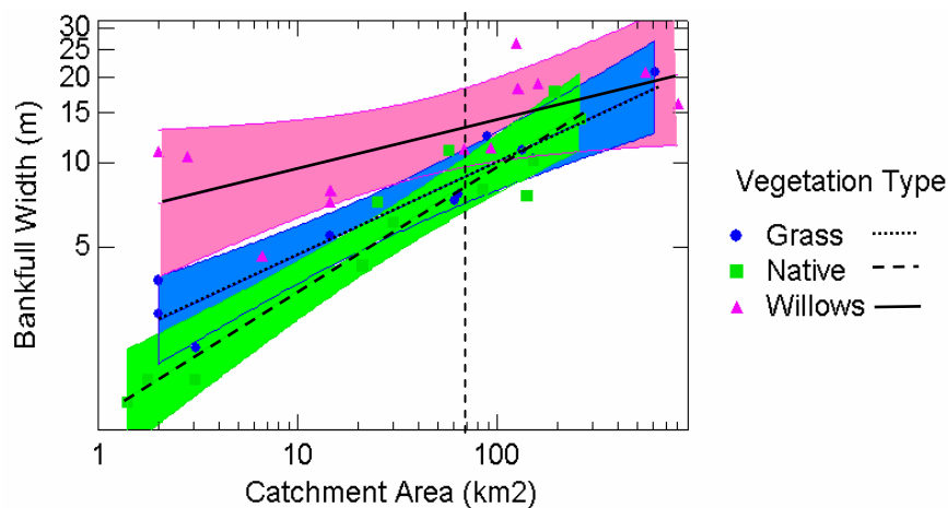
Figure 2. Scatter plot showing the relationship between vegetation type, bankfull width and catchment area (log-log scale). The shaded sections refer to the 95 percent confidence intervals around each regression line. The vertical dotted line indicates the point at which the confidence intervals of all three vegetation type overlap by more than a quarter (~70km 2 ).
