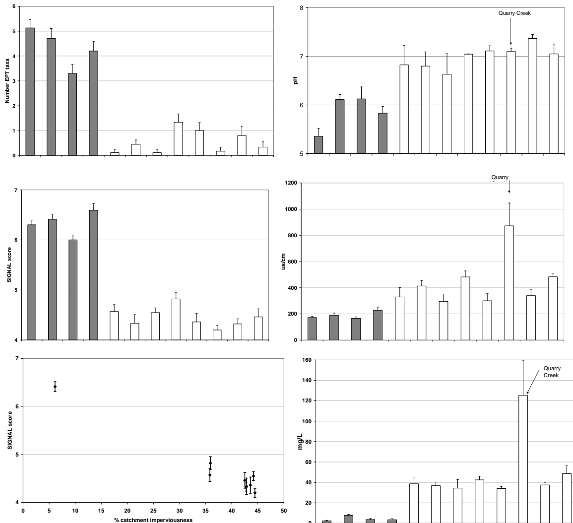
Figure 1. Macroinvertebrate (left) and water quality (right) results.
